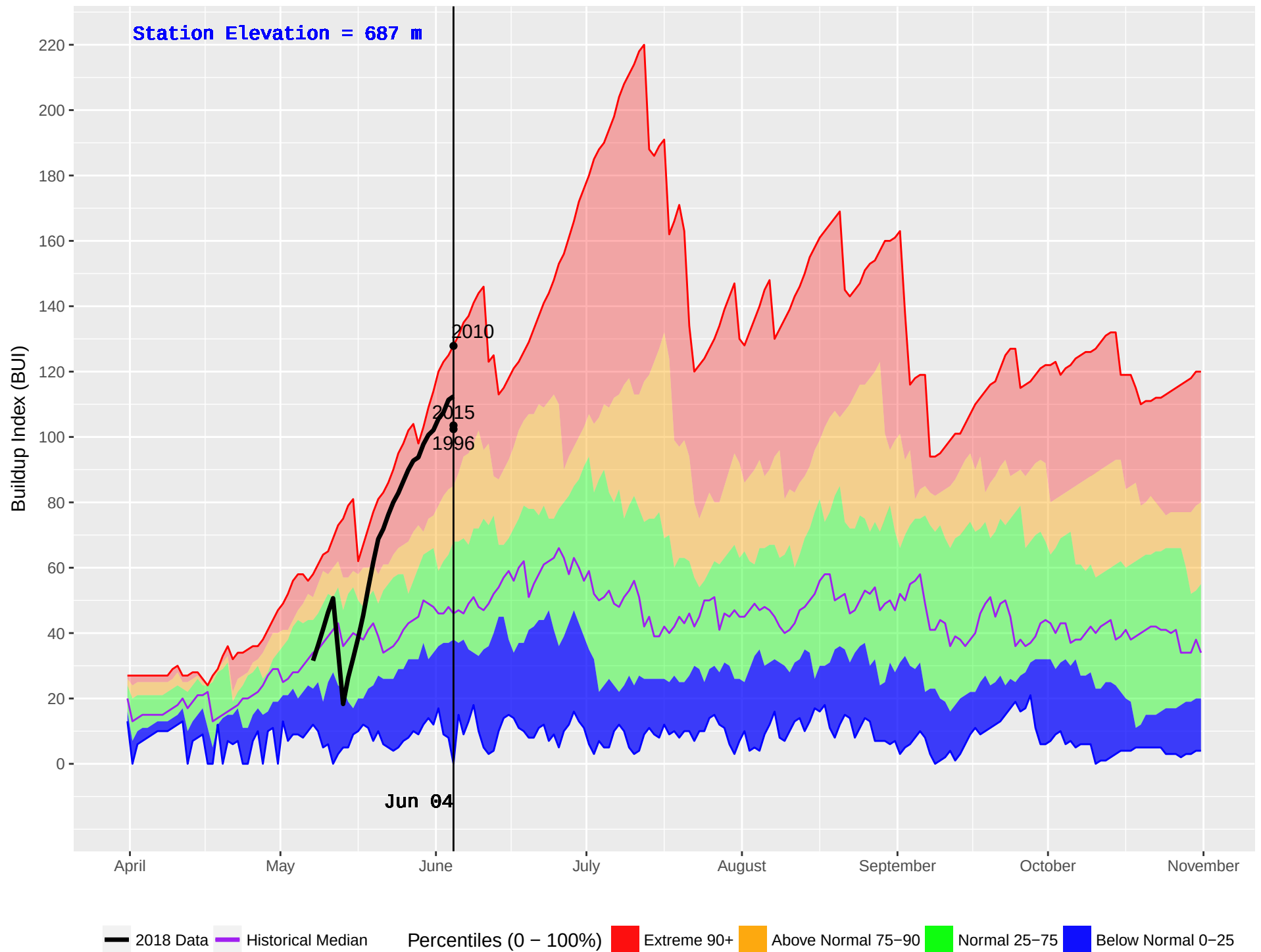
KETCHIKA (444) : Historical (1986–2016) and Current (2018) Noon Buildup Index (BUI)
