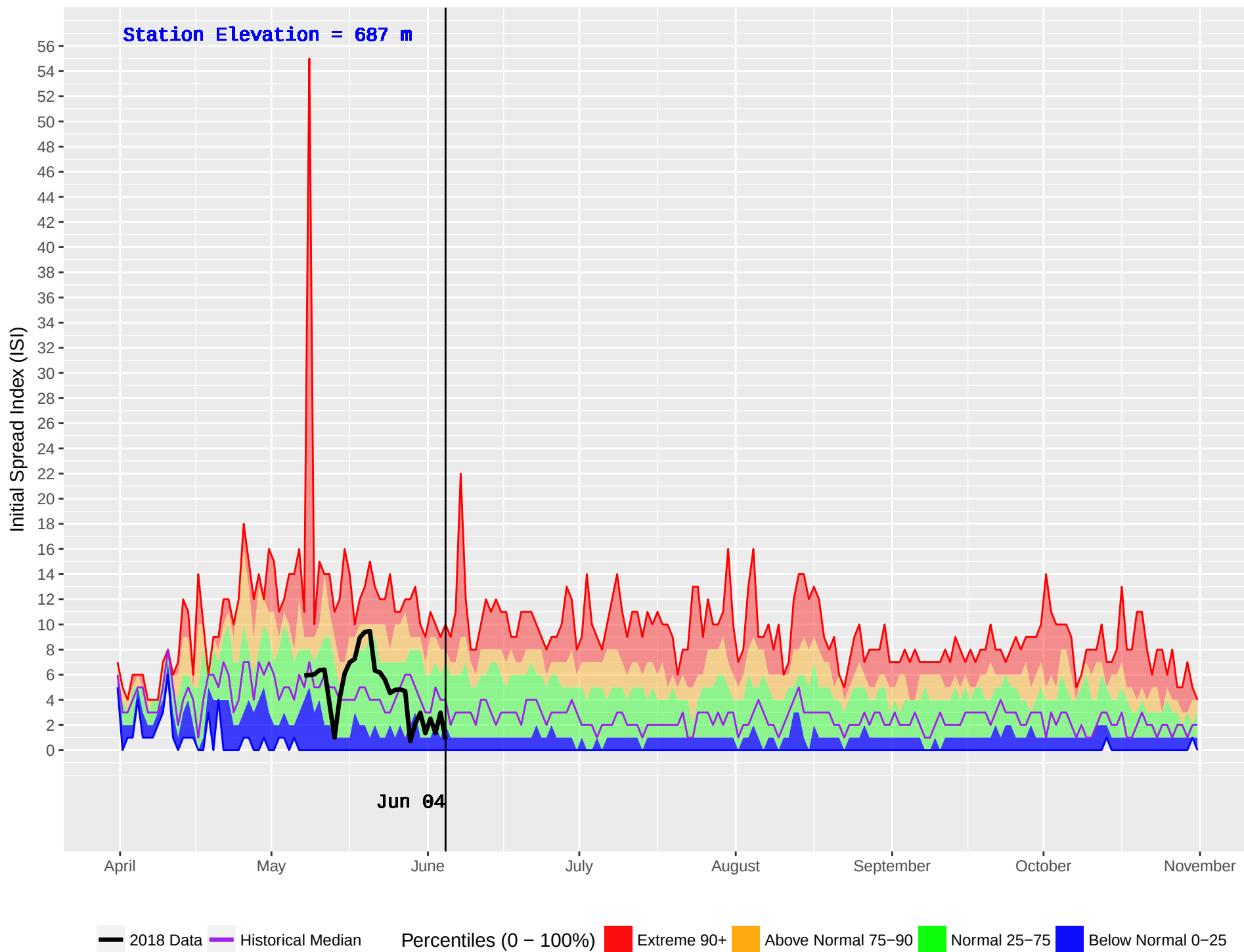
KETCHIKA (444) : Historical (1986–2016) and Current (2018) Noon Initial Spread Index (ISI)
