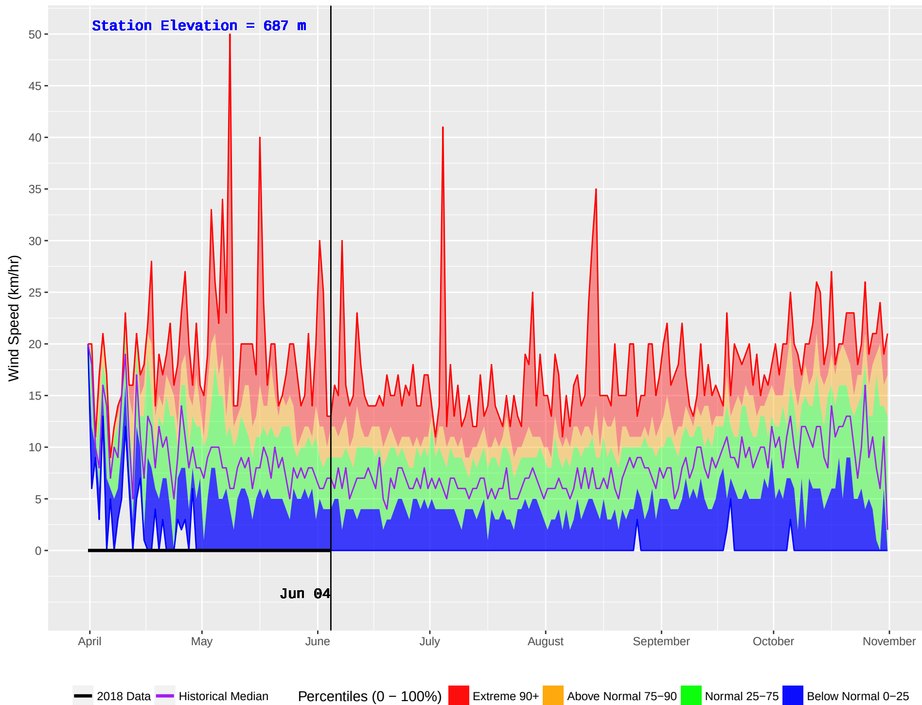
KETCHIKA (444) : Historical (1986–2016) and Current (2018) Noon Wind Speed
