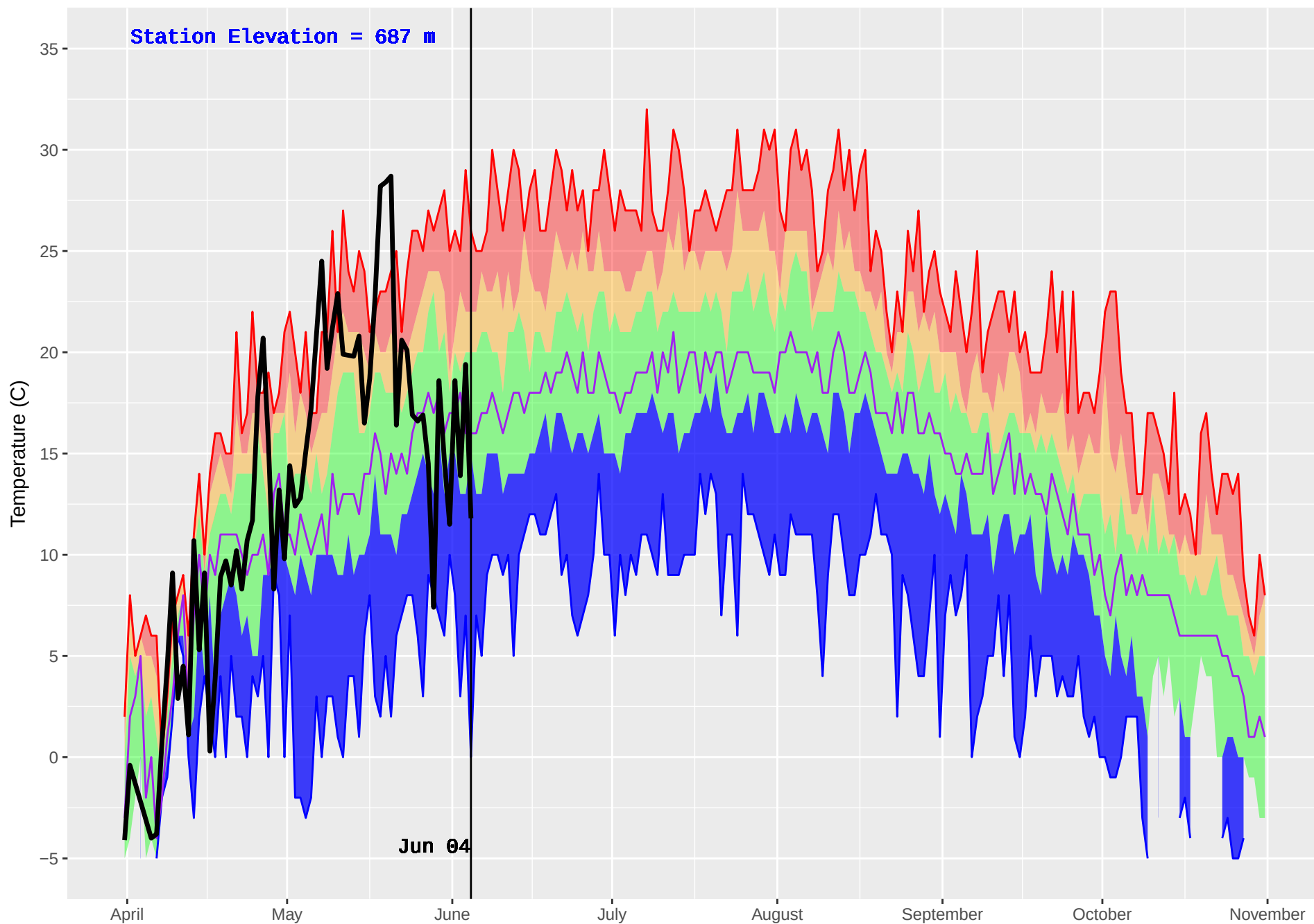
KETCHIKA (444) : Historical (1986–2016) and Current (2018) Noon Temperature
