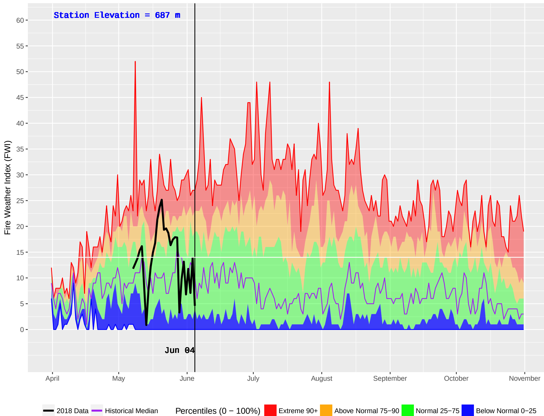
KETCHIKA (444) : Historical (1986–2016) and Current (2018) Noon Fire Weather Index (FWI)
