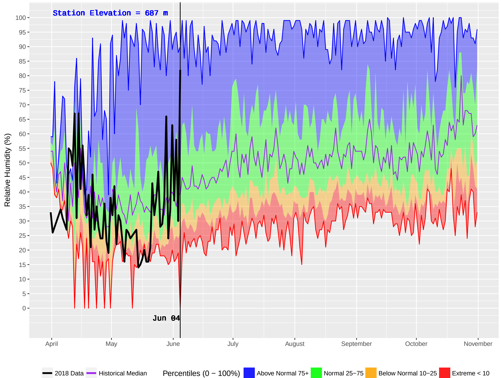
KETCHIKA (444) : Historical (1986–2016) and Current (2018) Noon Relative Humidity
