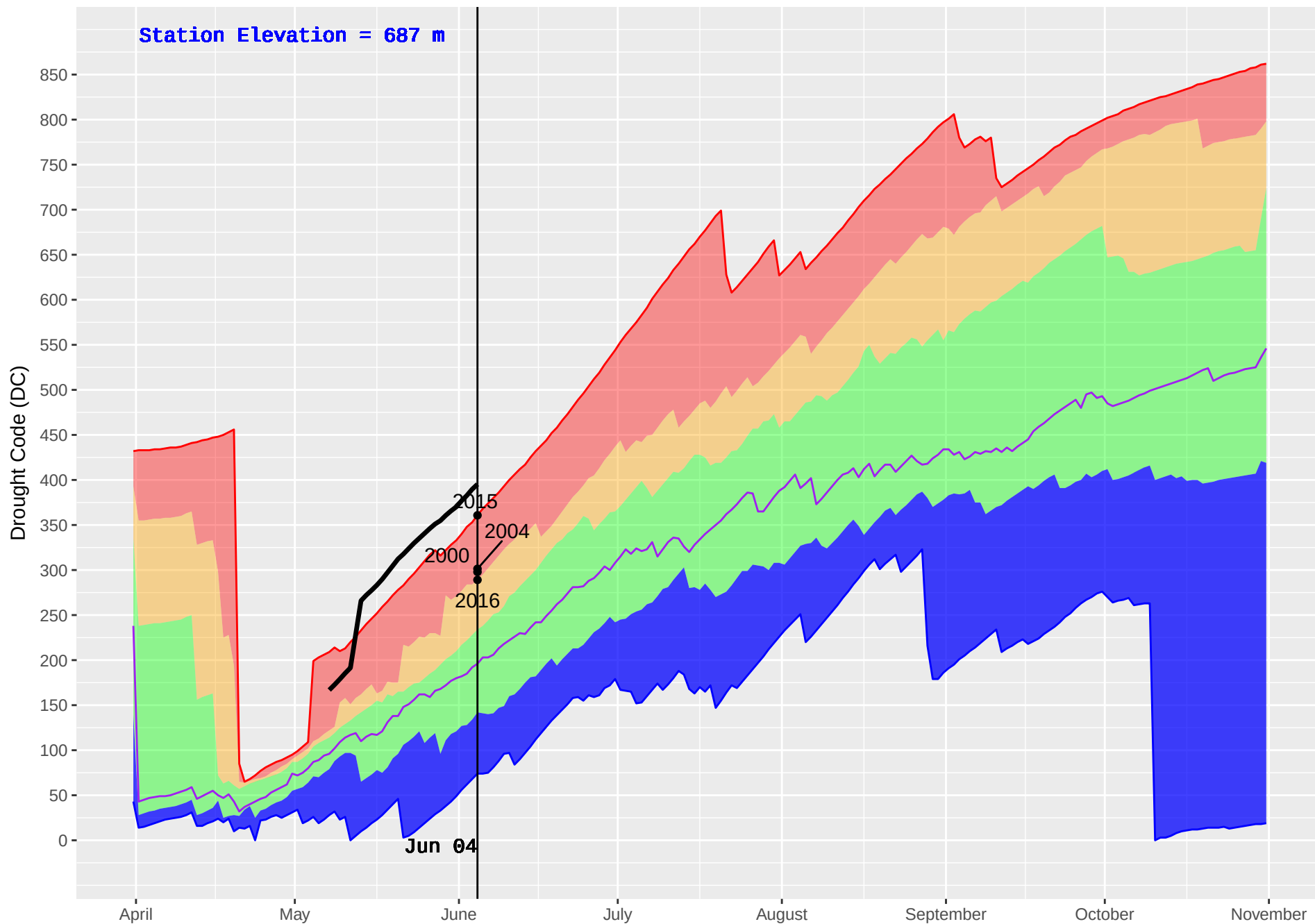
KETCHIKA (444) : Historical (1986–2016) and Current (2018) Noon Drought Code (DC)
