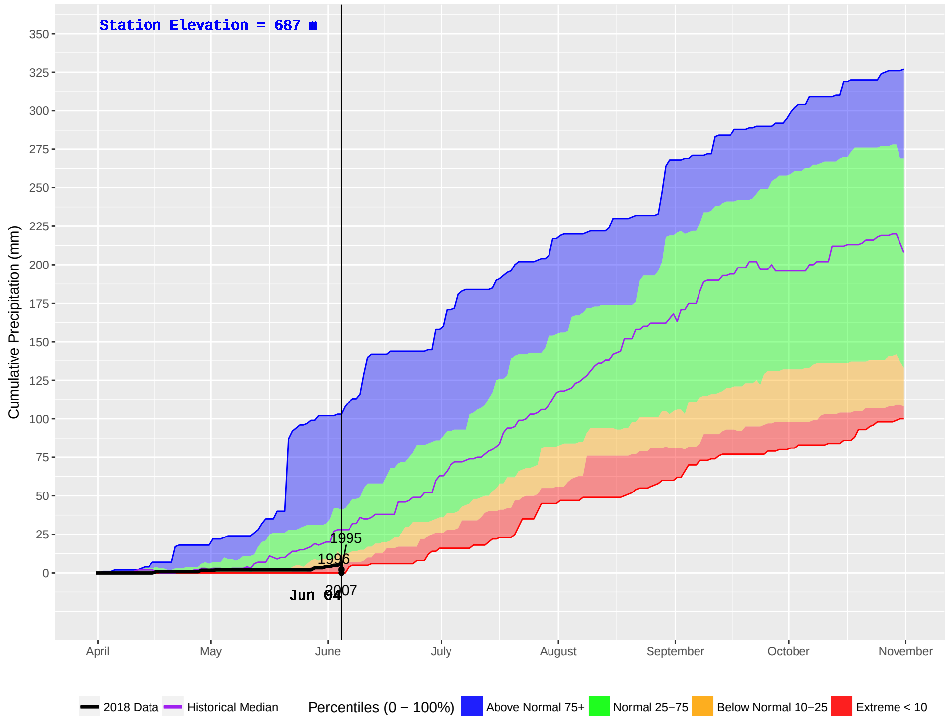
KETCHIKA (444) : Historical (1986–2016) and Current (2018) Noon Cumulative Precipitation
